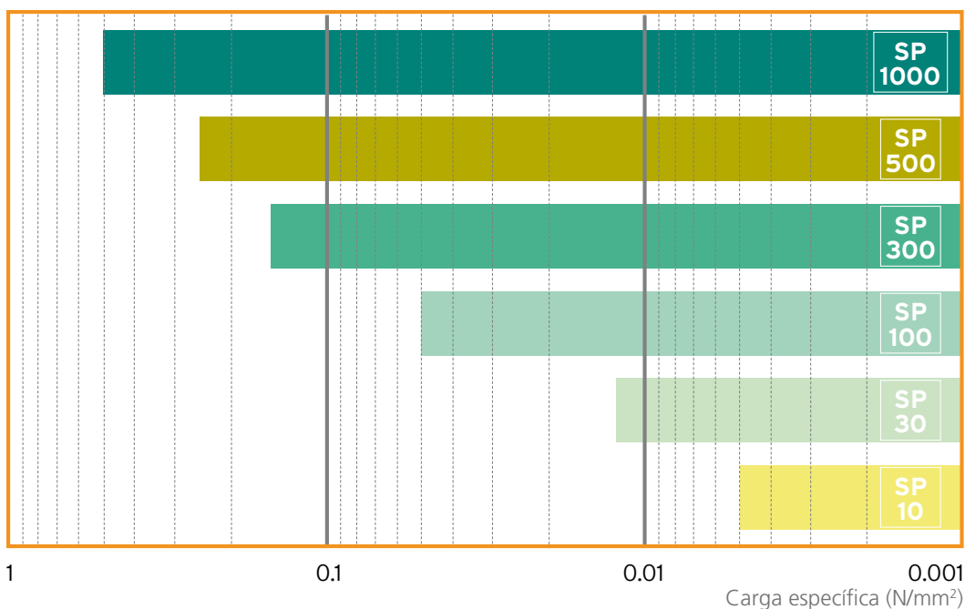
Fig. 1: Gama SyloDamp®
